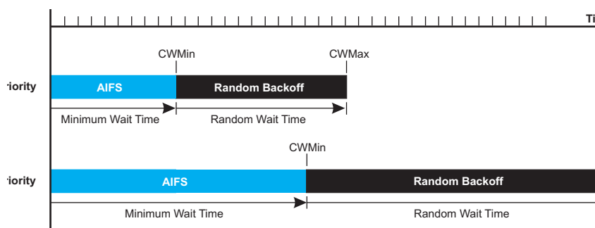
Figure 4-1. WMM Backoff Wait Times
