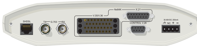
6541 Rear Panel
