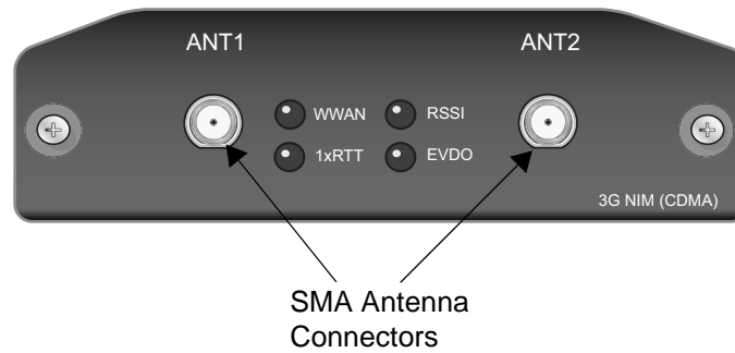
Figure 42. 3G CDMA NIM Rear Panel
