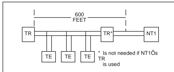
Figure B-1. Short Passive Bus Configuration
