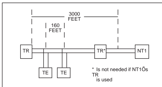
Figure B-2. Extended Passive Bus Configuration
