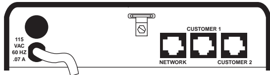
Figure 1-1. NT1 Type 400 Standalone Rear Panel
