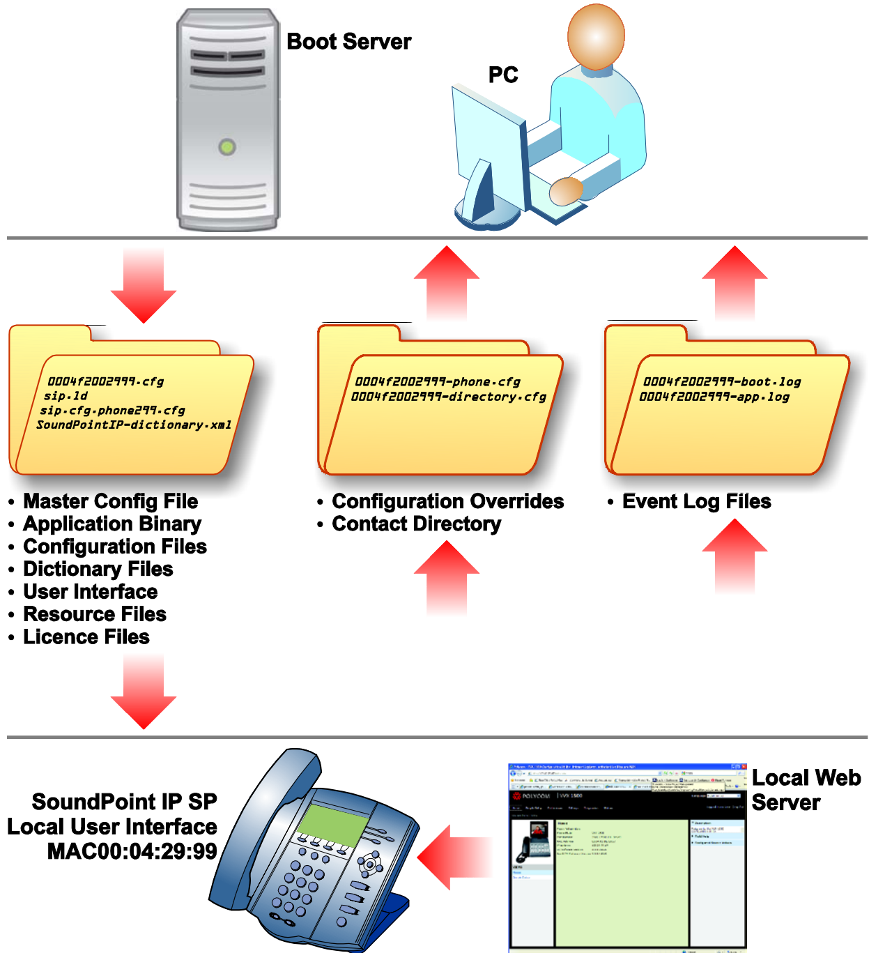
Figure 2-3: Network Layout Using Central Provisioning
