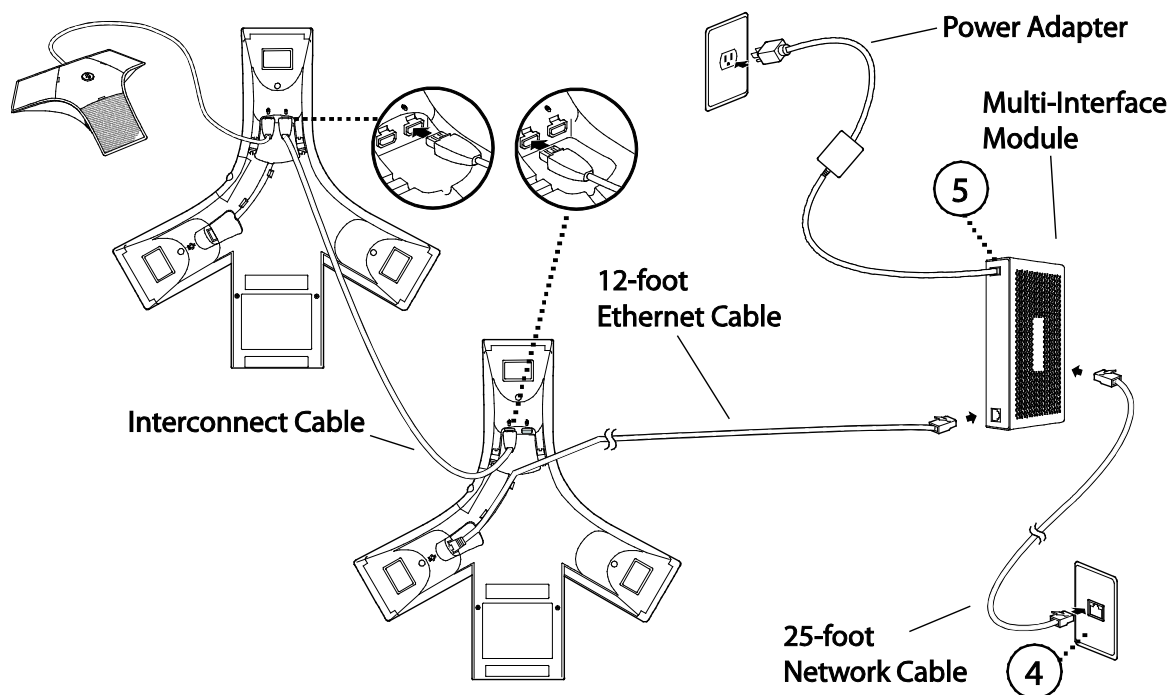
Figure 4-1: Daisy Chaining Two SoundStation IP 7000 Phones
