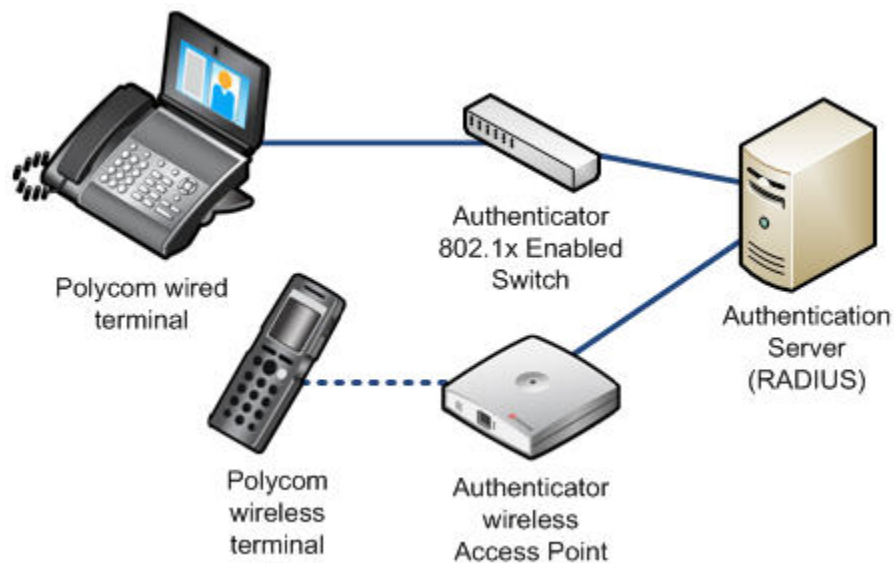
Figure 9-2: A Typical 802.1X Network Configuration
