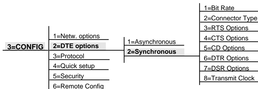
Figure 6-17 Synchronous DTE Options Menu Tree
