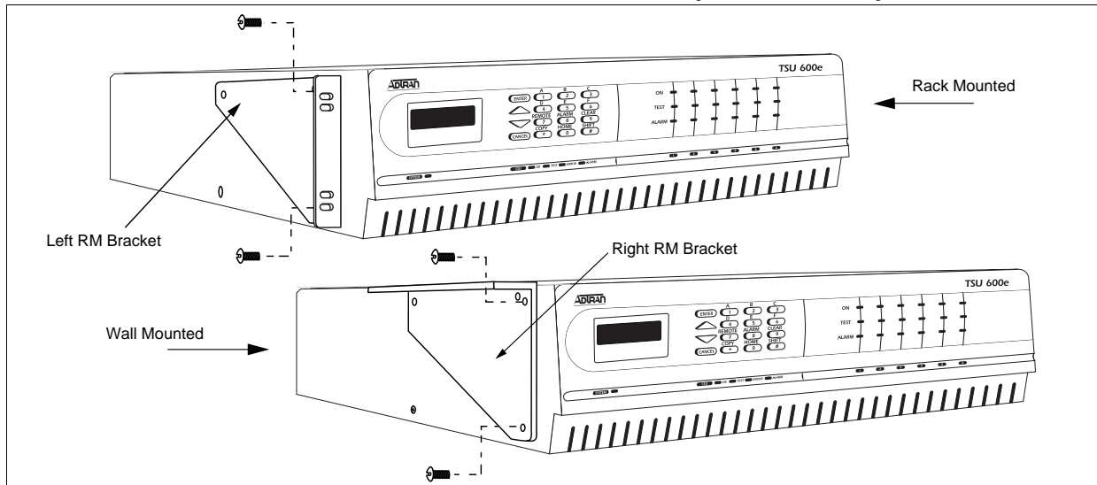
Figure 1. Installation of Rack Mount Brackets on a TSU 600e
